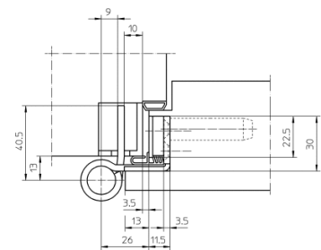
Blockzarge
